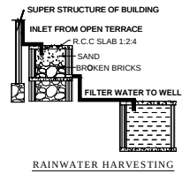
RAINWATER HARVESTING
