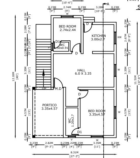
PRO.GROUND FLOOR
