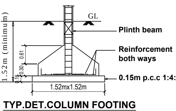
TYP.DET.COLUMN FOOTING
