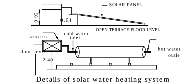
Details of solar water heating system
