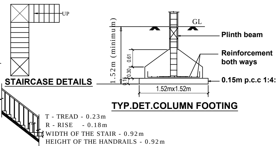
STAIRCASE DETAILS
