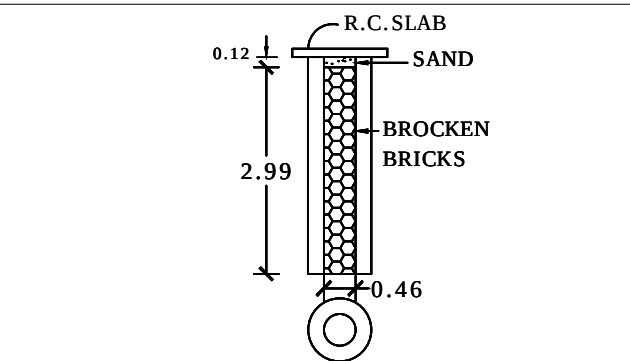
PERCOLATION PIT
