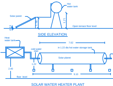
SOLAR WATER HEATER PLANT
