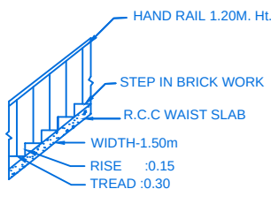
STAIR DETAIL
