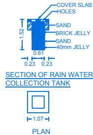
SECTION OF RAIN WATER COLLECTION TANK
