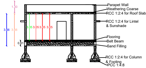
SECTION AB
