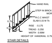
STAIR DETAILS
