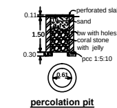
percolation pit
