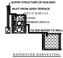
RAINWATER HARVESTING
