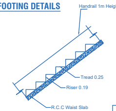
STAIR DETAILS
