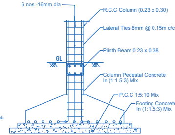
COLUMN FOOTING DETAILS
