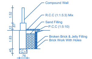
RAIN WATER HARVEST DETAILS
