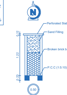
RAIN WATER COLLECTION WELL
