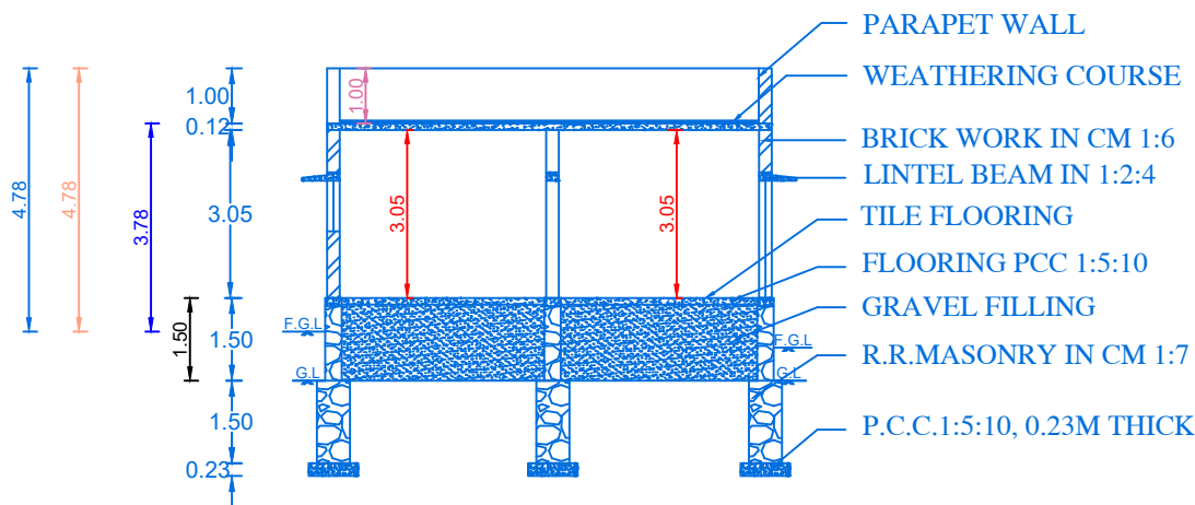
SECTION ON "V-B"
