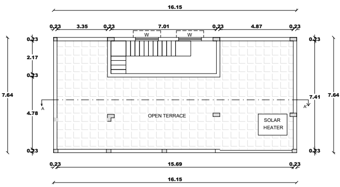
HEAD ROOM & OPEN TERRACE FLOOR PLAN
