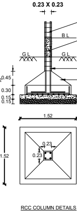
RCC COLUMN DETAILS
