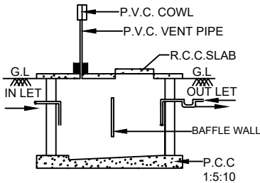
SEC. OF SEPTIC TANK
