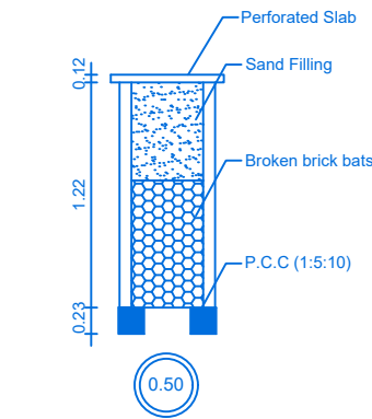
RAIN WATER COLLECTION WELL
