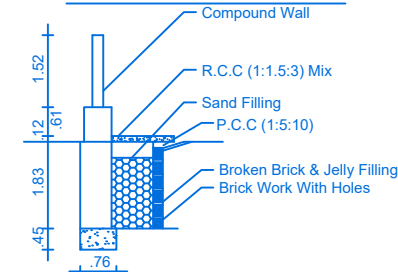
RAIN WATER HARVEST DETAILS
