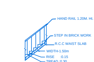
STAIR DETAIL
