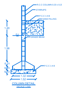
COLUMN DETAIL
