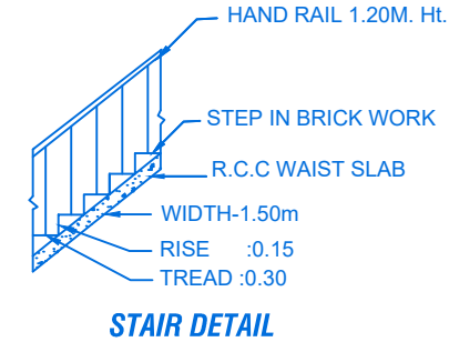
STAIR DETAIL
