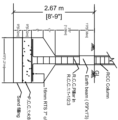
FOUNDATION DETAILS
