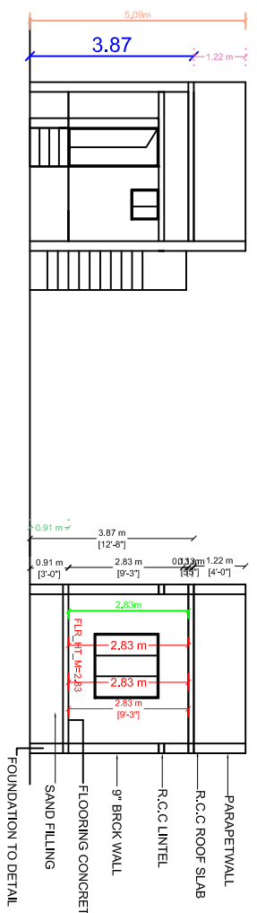
FRONT ELEVATION
