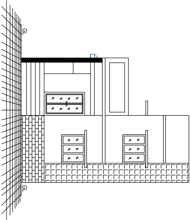
FRONT ELEVATION
