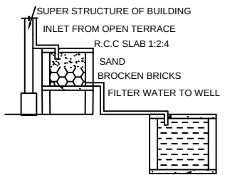
RAINWATER HARVESTING
