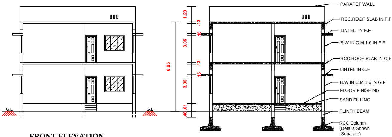
CROSS SECTION VIEW AB
