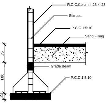
COLUMN DETAIL
