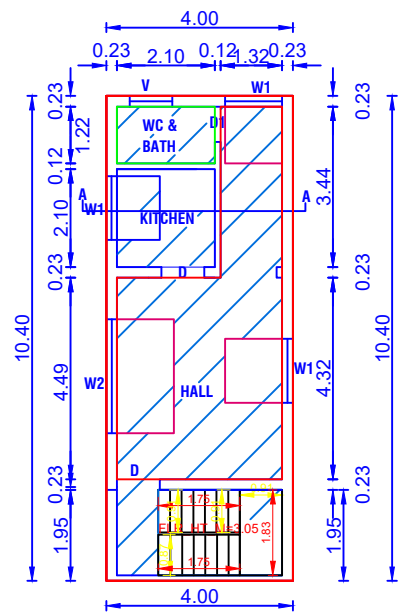
GROUND FLOOR PLAN(EXISTING BUILDING)
