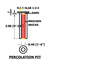
PERCOLATION PIT
