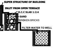
RAINWATER HARVESTING
