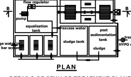
DETAILS OF SEWAGE TREATMENT PLANT
