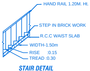
STAIR DETAIL
