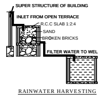
RAINWATER HARVESTING
