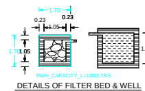
DETAILS OF FILTER BED & WELL
