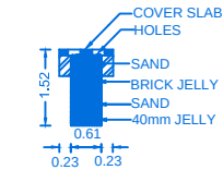
SECTION OF RAIN WATER COLLECTION TANK
