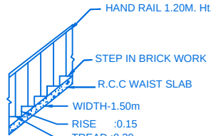
STAIR DETAIL
