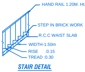
STAIR DETAIL
