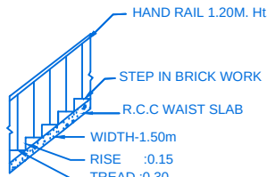
STAIR DETAIL
