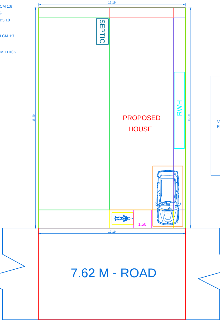
SEPTIC TANK AND TRENCH & U TRAP ADOPTED
