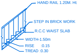
STAIR DETAIL
