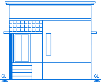
FRONT ELEVATION
