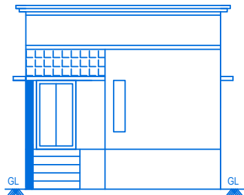
FRONT ELEVATION
