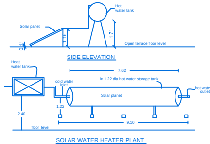
SIDE ELEVATION
