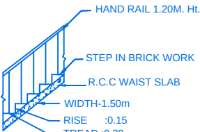
STAIR DETAIL
