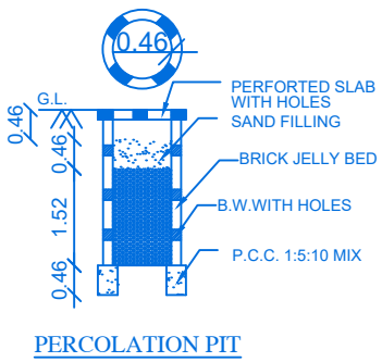
PERCOLATION PIT
