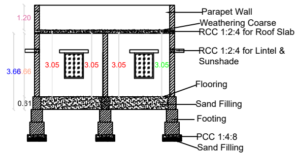
SECTION AB
