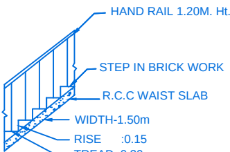
STAIR DETAIL
