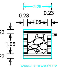
DETAILS OF FILTER BED & WELL
