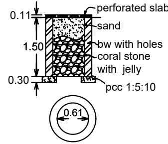
percolation pit
