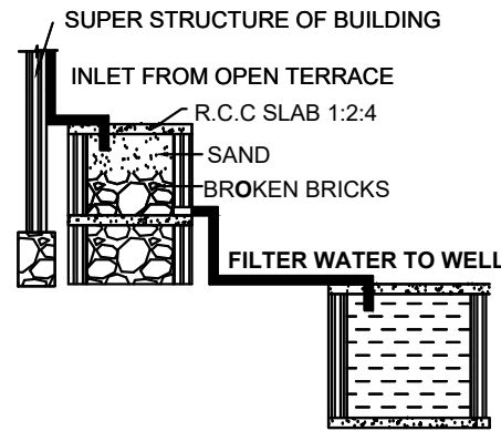
RAINWATER HARVESTING
