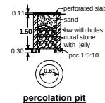
percolation pit
