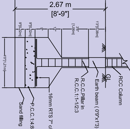
FOUNDATION DETAILS
