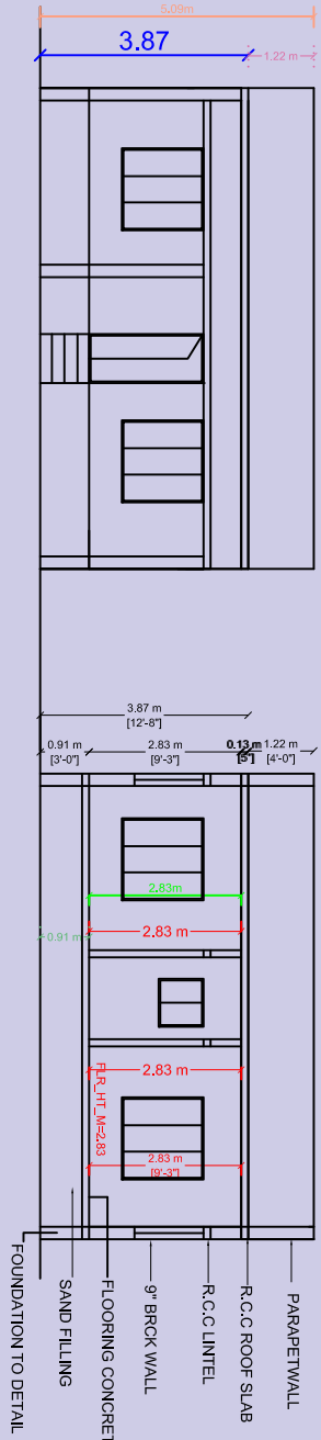
FRONT ELEVATION
