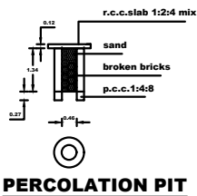
PERCOLATION PIT
