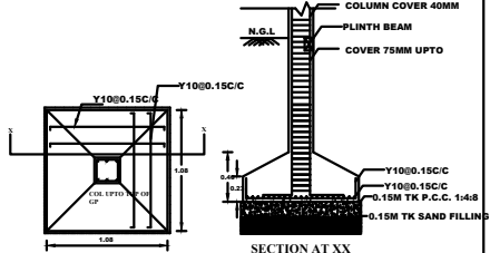
SECTION AT XX
