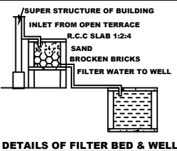
DETAILS OF FILTER BED & WELL
