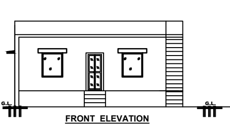
FRONT ELEVATION
