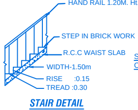
STAIR DETAIL
