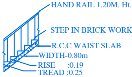
STAIR DETAIL
