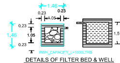
DETAILS OF FILTER BED & WELL
