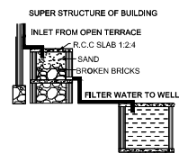
RAINWATER HARVESTING
