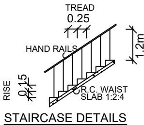
STAIRCASE DETAILS
