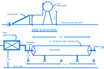
SOLAR WATER HEATER PLANT
