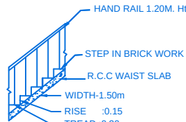
STAIR DETAIL
