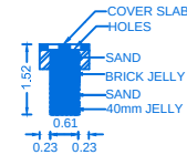
SECTION OF RAIN WATER COLLECTION TANK
