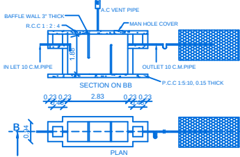
SEPTIC TANK AND TRENCH & U TRAP ADOPTED
