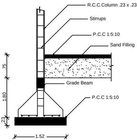
COLUMN DETAIL
