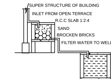
RAINWATER HARVESTING
