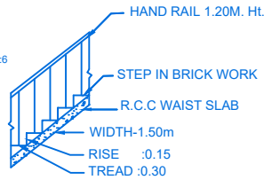
STAIR DETAIL
