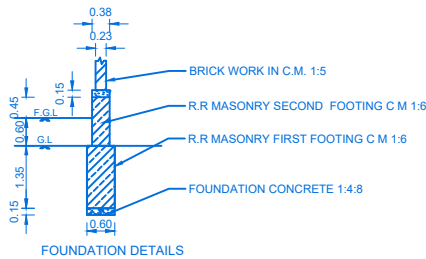
FOUNDATION DETAILS
