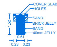
SECTION OF RAIN WATER COLLECTION TANK
