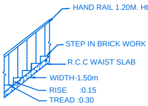
STAIR DETAIL
