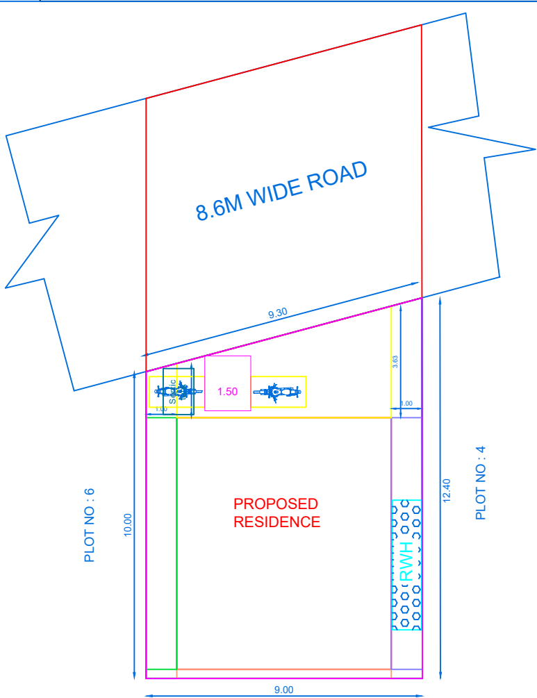
SITE PLAN
