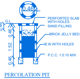
PERCOLATION PIT
