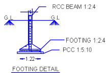
FOOTING DETAIL
