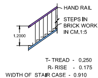
DETAILS OF STAIRCASE
