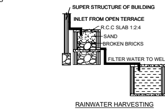
RAINWATER HARVESTING
