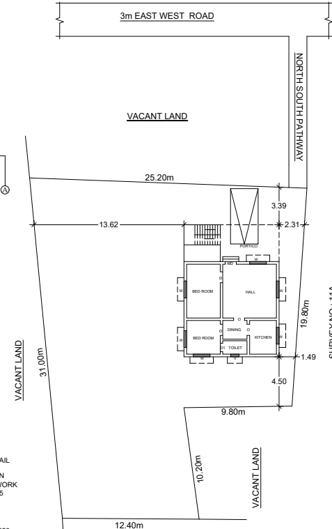
SURVEY NO : 258/1B SITE PLAN SCALE (1:200)
