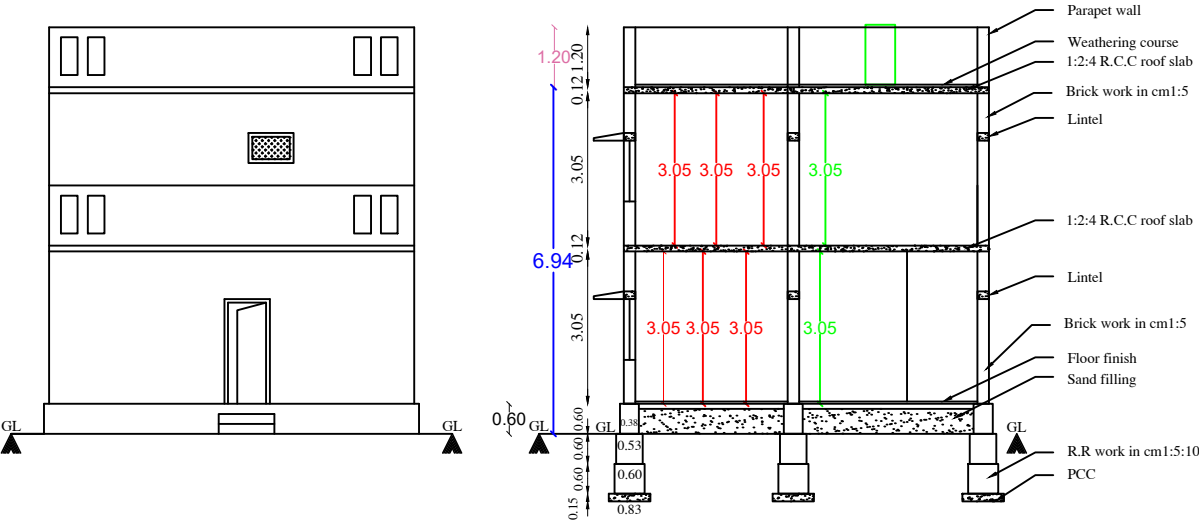
FRONT ELEVATION
