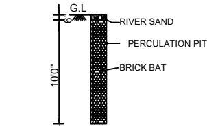
PERCOLATION PIT
