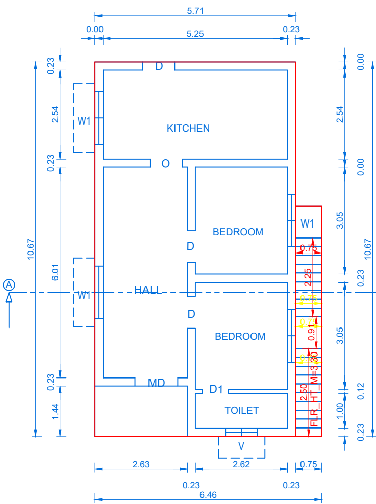
EXT.GROUND FLOOR PLAN
