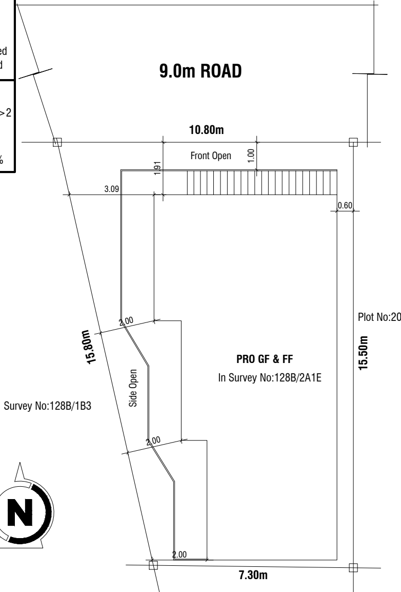
SITE PLAN
