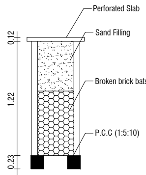
RAIN WATER COLLECTION WELL
