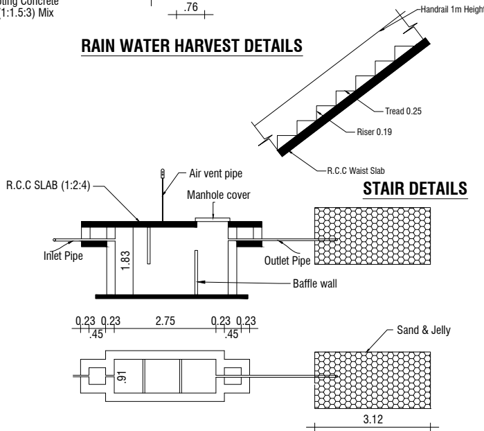
SEPTIC TANK & TRENCH
