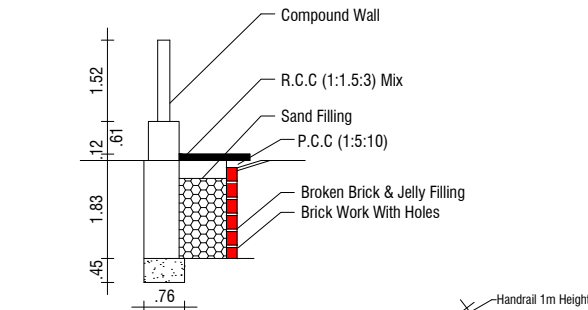
RAIN WATER HARVEST DETAILS
